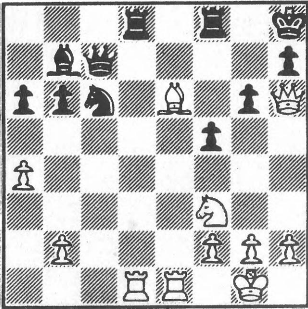
202 After 20...Rad8
